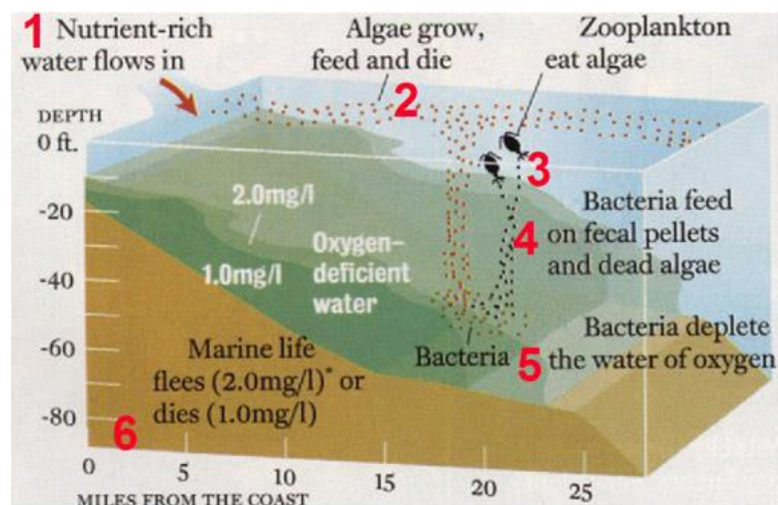
Fig. 2-7. Schematic depicting the evolution of hypoxia in coastal waters. Source: Gulfhypoxia.net
